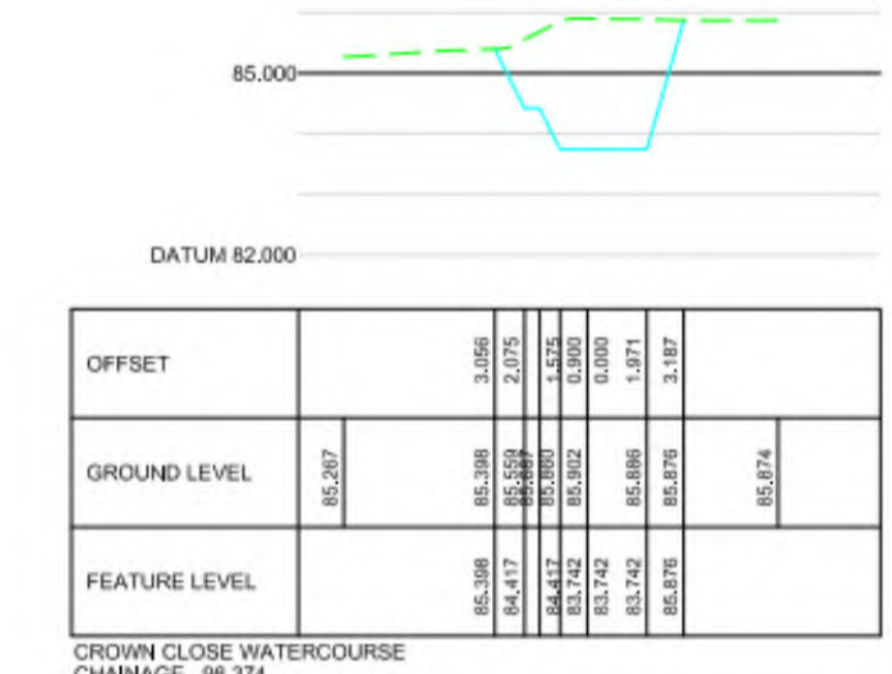
CROWN CLOSE WATERCOURSE CHAINAGE 96.374
