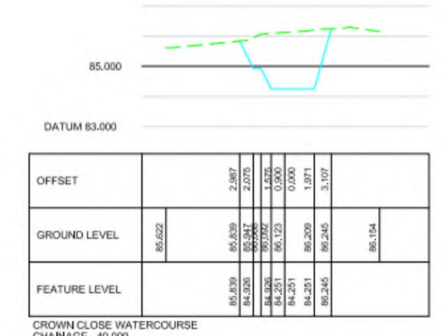
CROWN CLOSE WATERCOURSE CHAINAGE 80.000
