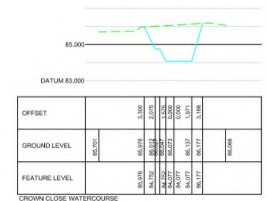
CROWN CLOSE WATERCOURSE CHAINAGE 60.000
