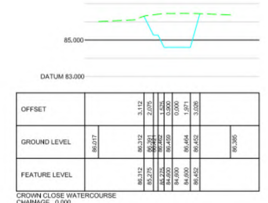
CROWN CLOSE WATERCOURSE CHAINAGE 40.000
