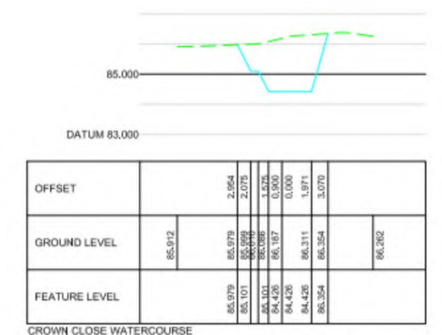
CROWN CLOSE WATERCOURSE CHAINAGE 20.000
