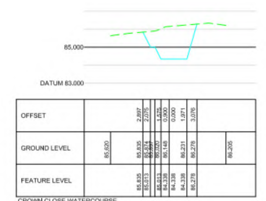
CROWN CLOSE WATERCOURSE CHAINAGE 30.000
