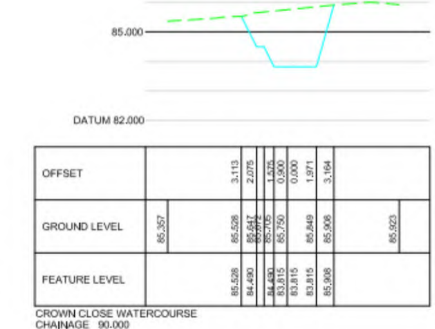
CROWN CLOSE WATERCOURSE CHAINAGE 90.000
