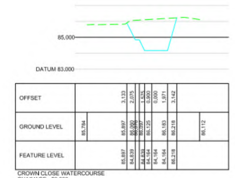
CROWN CLOSE WATERCOURSE CHAINAGE 50.000
