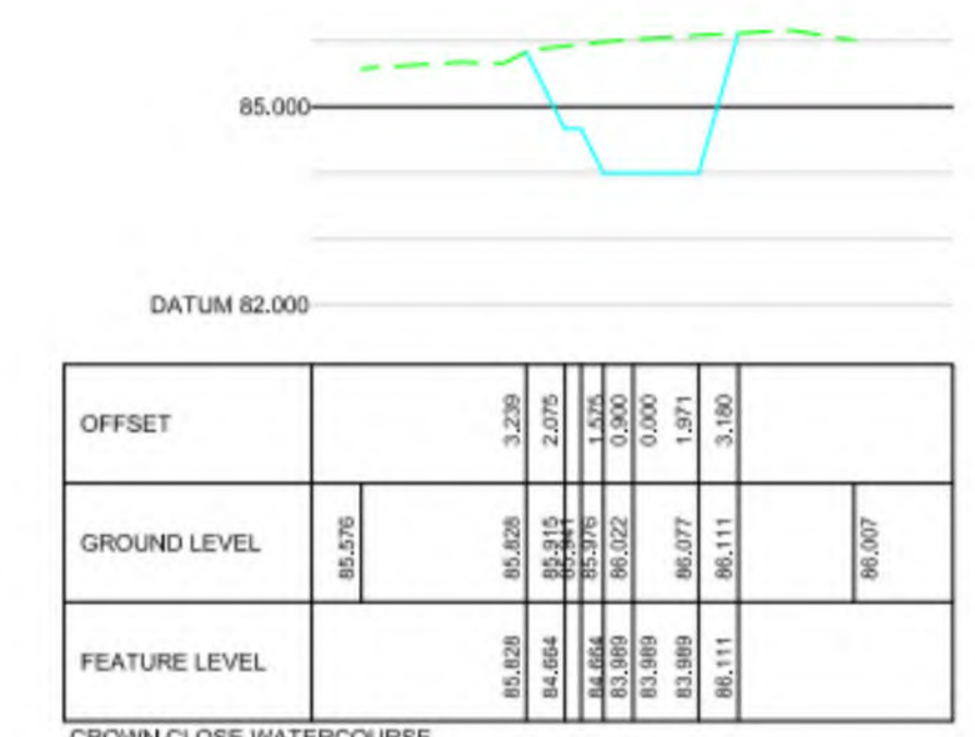
CROWN CLOSE WATERCOURSE CHAINAGE 70.000
