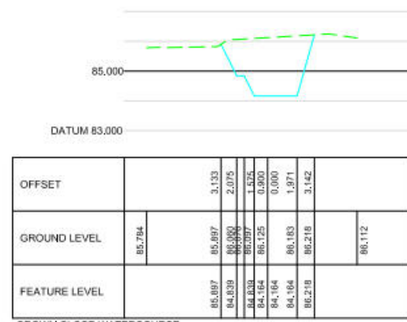
CROWN CLOSE WATERCOURSE CHAINAGE 50.000
