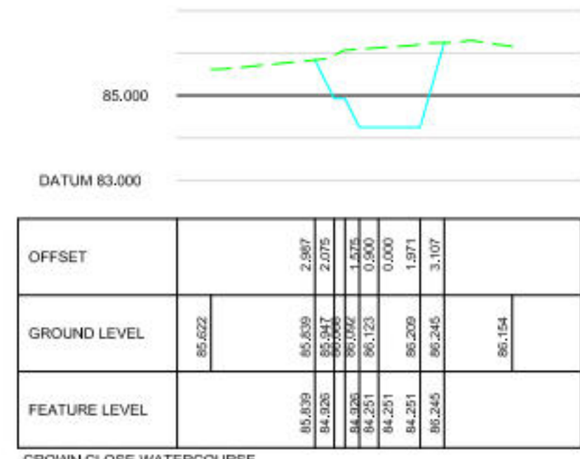
CROWN CLOSE WATERCOURSE CHAINAGE 40.000
