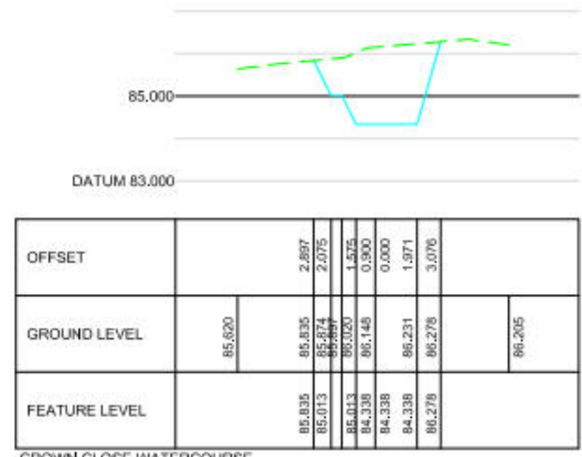
CROWN CLOSE WATERCOURSE CHAINAGE 30.000
