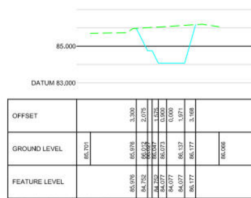
CROWN CLOSE WATERCOURSE CHAINAGE 60.000
