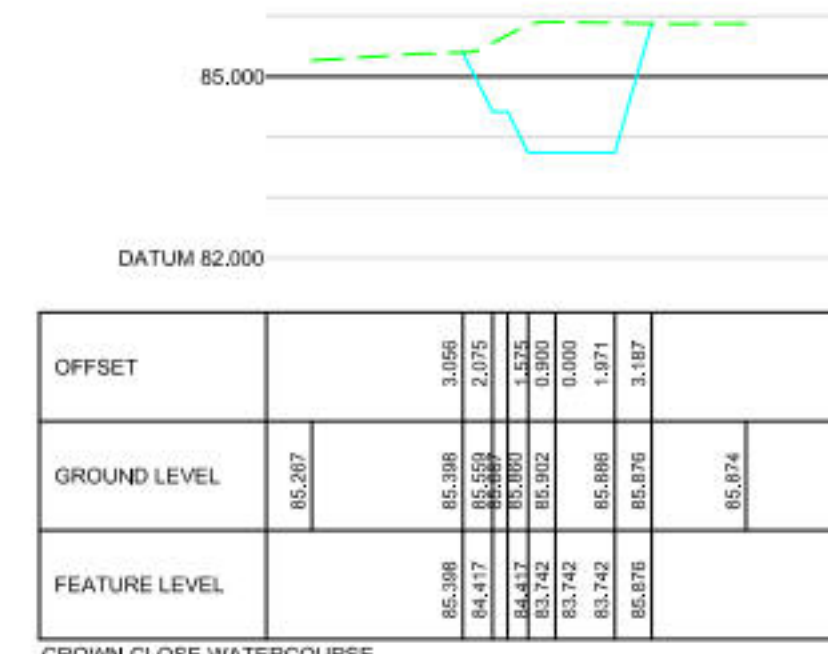
CROWN CLOSE WATERCOURSE CHAINAGE 96.374
