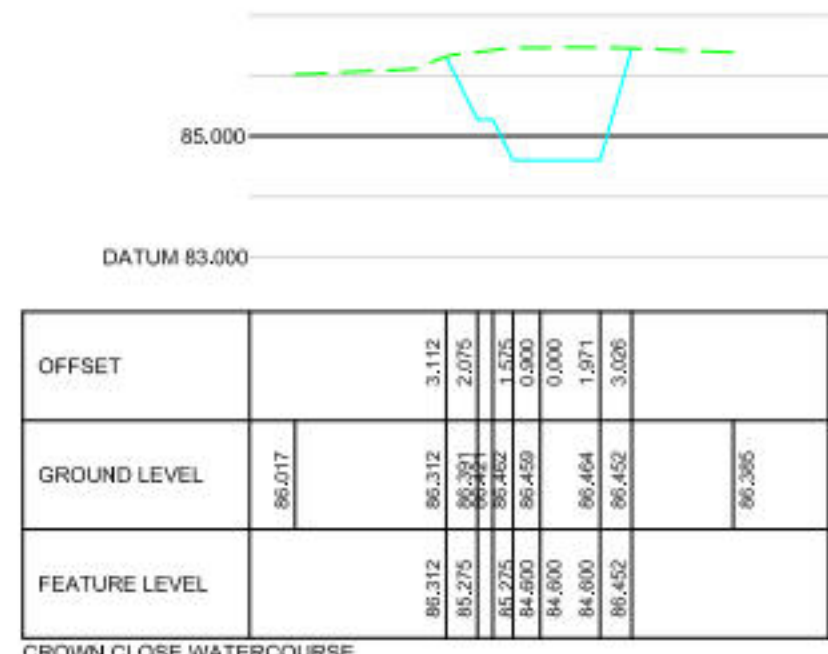
CROWN CLOSE WATERCOURSE CHAINAGE 0.000
