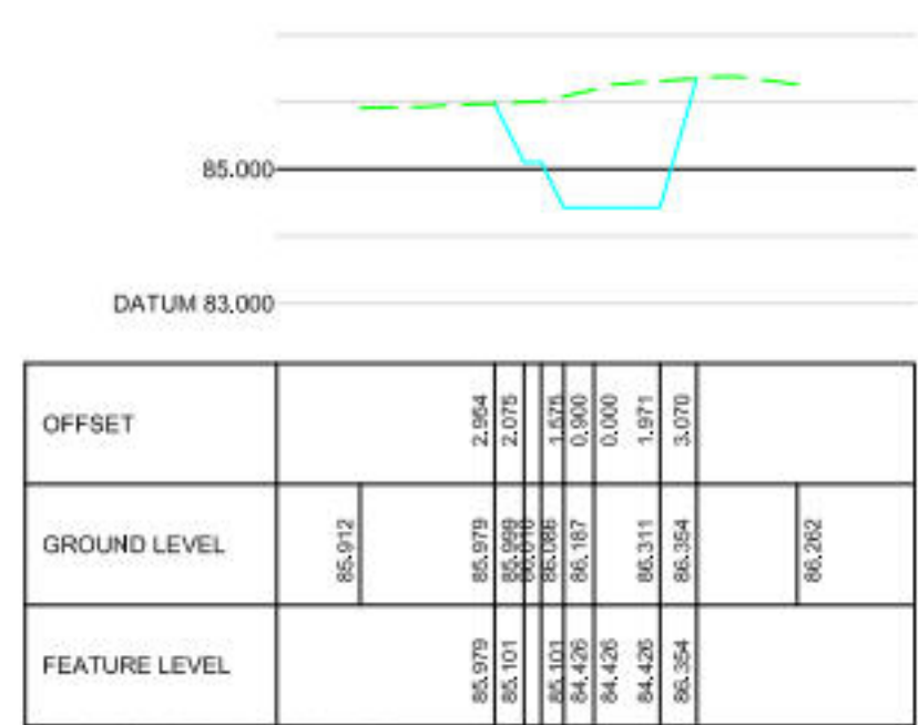
CROWN CLOSE WATERCOURSE CHAINAGE 20.000
