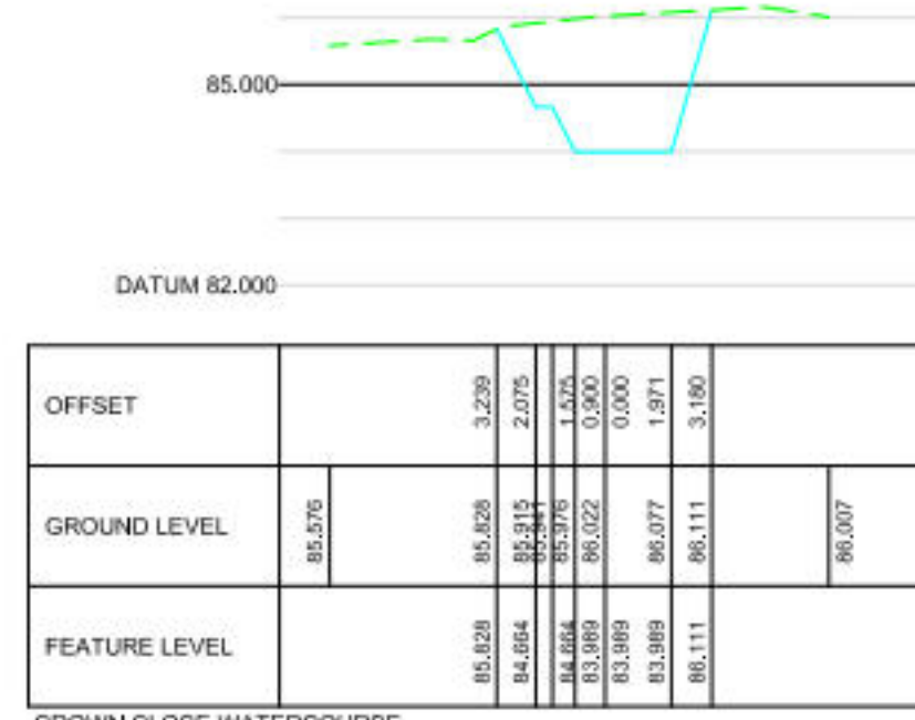
CROWN CLOSE WATERCOURSE CHAINAGE 70.000
